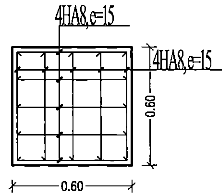
Footing
