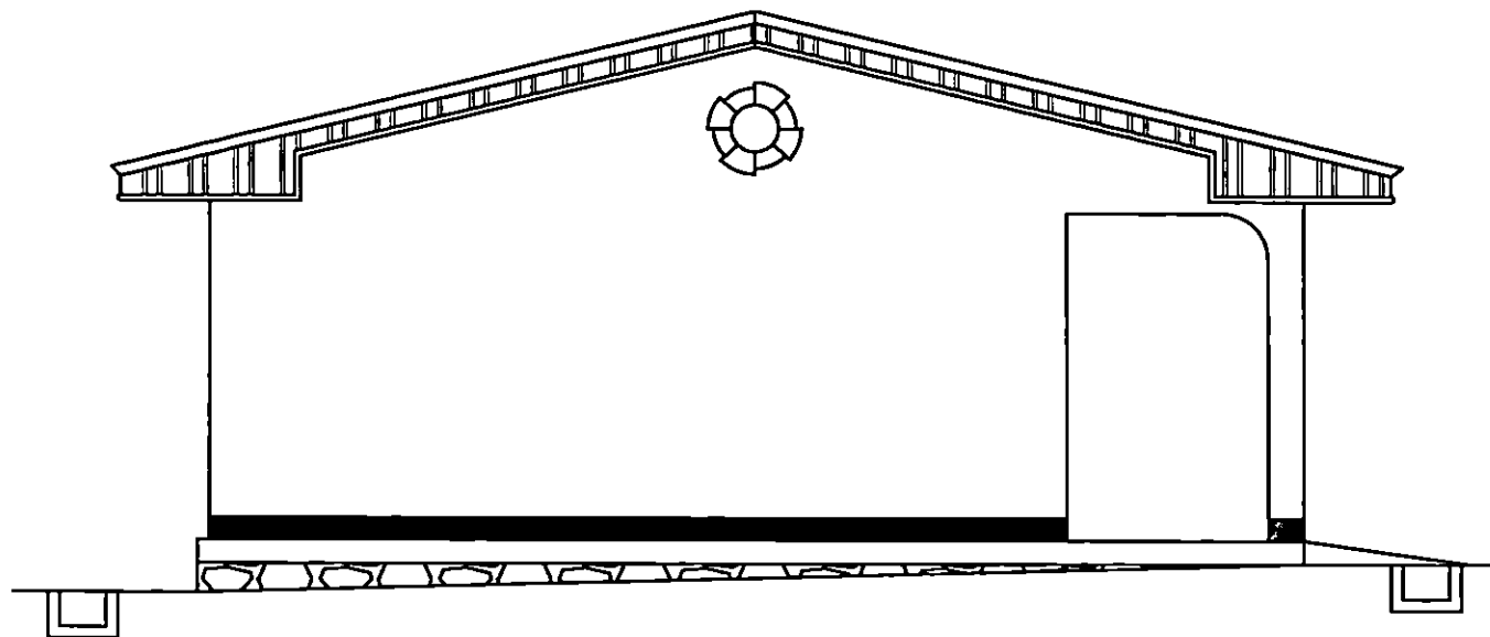
LEFT VIEW
