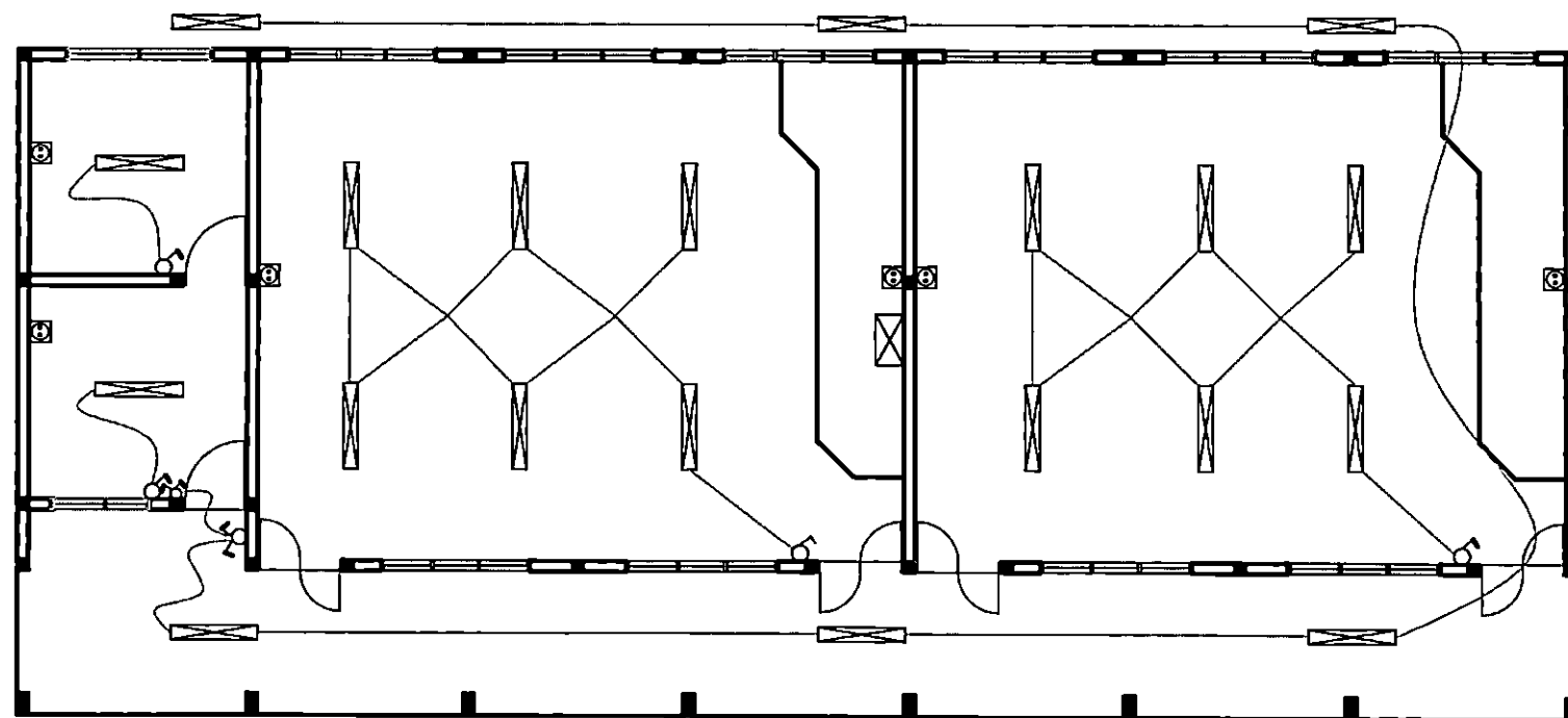
ELECTRICAL PLAN
