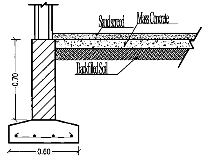
Foundation
