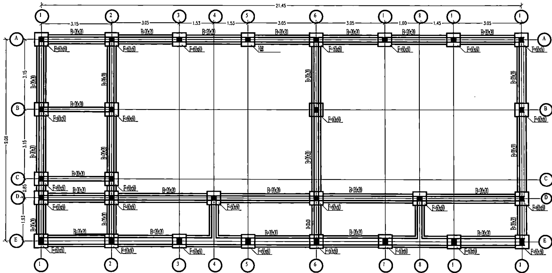
FOUNDATION PLAN
