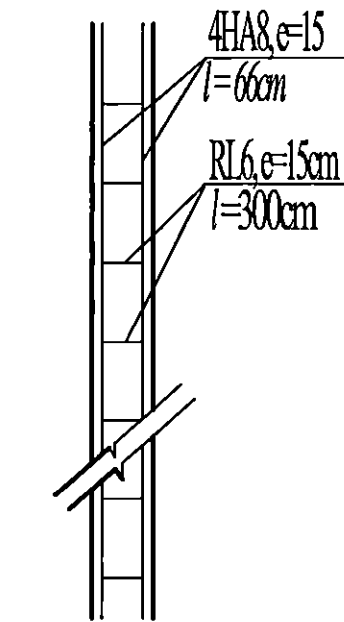
Pillar
