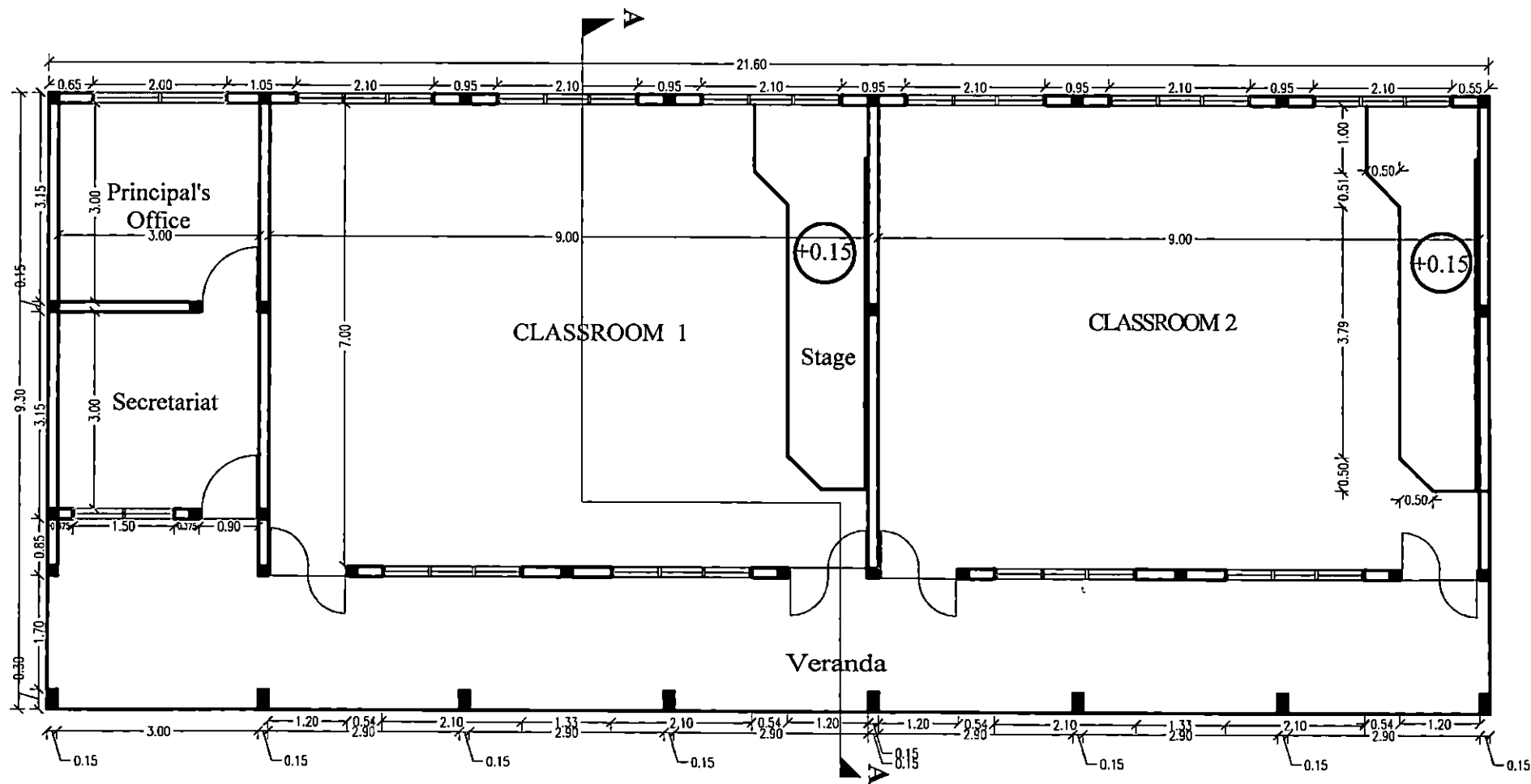
DISTRIBUTION PLAN
